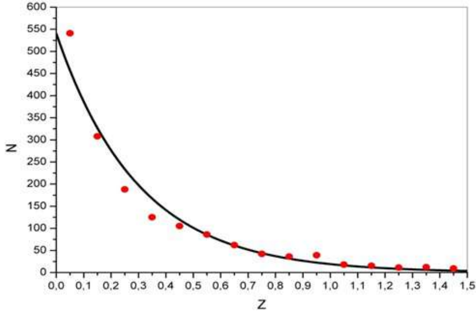
Figure 3. Distribution of absolute values of pulsar distances from the Galactic plane.
